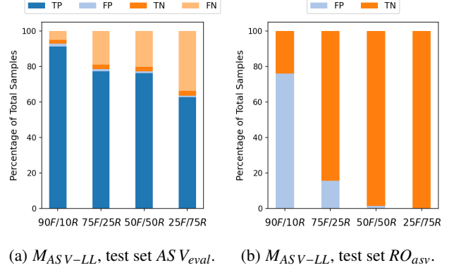
Figure 2: To show bias in the training and test sets of deepfake datasets, we examine M_{ASV-LL} with four different training distributions. Note the reduction in true positives, and consequently, the reduction in false positives. Results for M_{ASV-RN} , M_{ASV-SW} , M_{CFAD-RN} , and M_{CFAD-LL} may be found on our companion website, Figure 10 and Figure 11.
