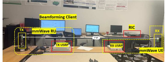
Fig. 1. Overview of the Milli-O-RAN testbed.
