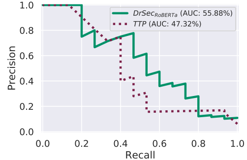
Figure 8: Alert-triage PR curves on Dsoc , when training on 50% of the training split. The AUCs are reported in the legend.
