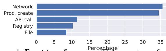
Figure 1: Event-type frequency. The percentage of events belonging to each event type in D Large .
