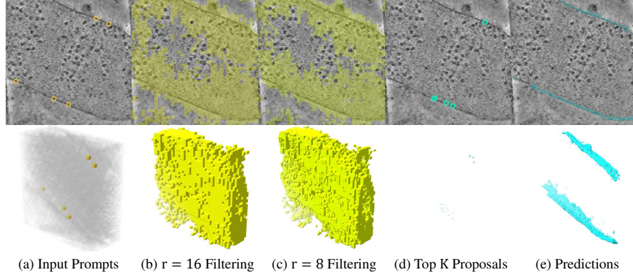
Fig. 7. Intermediate and final predictions of CryoSAM for membrane segmentation. CryoSAM can segment membranes with sparse prompt inputs.
