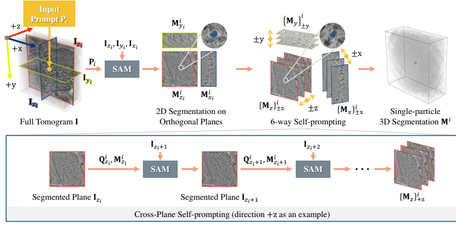
Fig. 2. The pipeline of prompt-based 3D segmentation. After segmenting the orthogonal planes intersect at the point prompt P_i , we iteratively execute Cross-Plane Self-Prompting until we get the complete mask of the particle.
