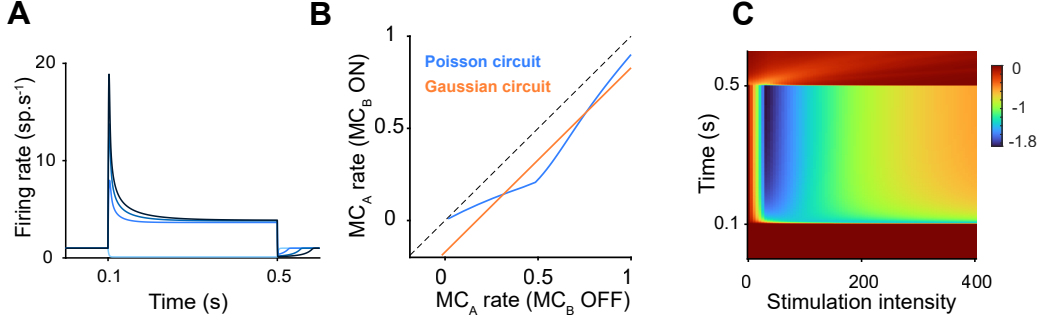
Figure 2: State-dependent inhibition of mitral cells. A. Upon stimulation, mitral cells exhibit a transient burst of activity followed by relaxation to a plateau. Darker color indicates stronger stimulation. B. In the circuit for Poisson CS we propose (blue line), the inhibition due to the activation of a second mitral cell ( MC_B ) is gated by the activity of the cell we are recording from ( MC_A ), as observed experimentally by Arevian et al. [95] in their Fig. 2D. This state-dependent gating does not occur in a circuit derived from a Gaussian noise model (orange line). Rates are normalized to the maximal stimulation of the principal cell. Dashed line indicates the unity line. C. Strength of inhibition as a function of time and of stimulation intensity; c.f. [95] Fig. 3B.
