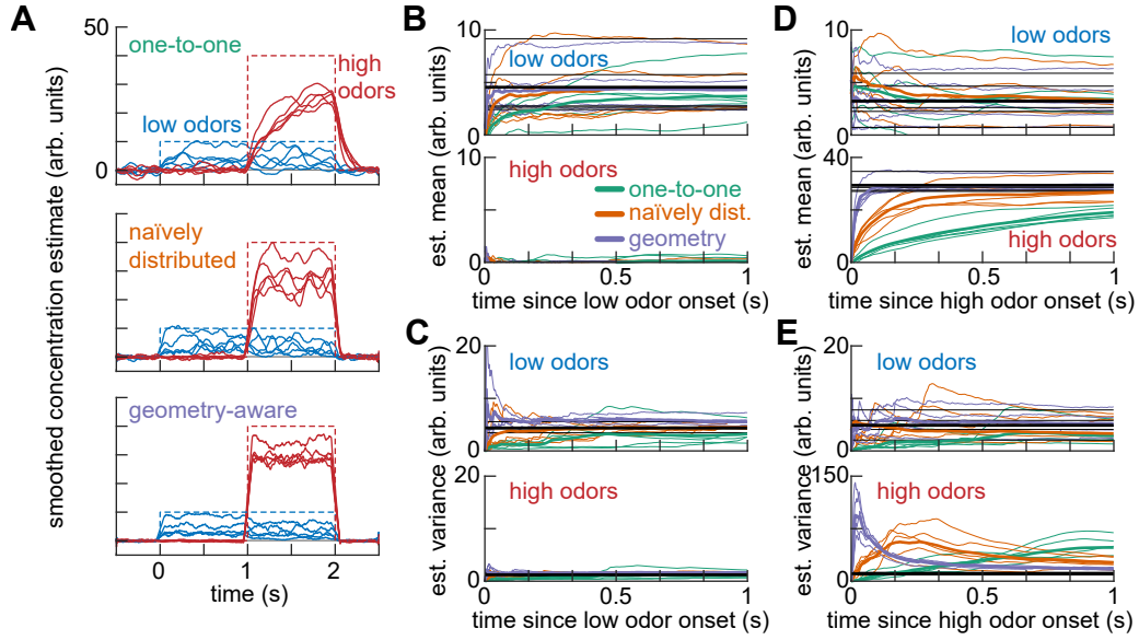
Figure G.3: Fast uncertainty estimation using Langevin sampling of the posterior, showing estimates for individual odorants. Here, we use a simple concentration estimation task in which 5 randomly-selected ‘low’ odorants out of a panel of 1000 appear at concentration 10 at time 0 s, and then a further 5 randomly-selected ‘high’ odorants appear at concentration 40 at time 1 s. A. Smoothed timeseries of instantaneous concentration estimates for low , high , and background odorants, for models with one-to-one ( top ), naively distributed ( middle ), and geometry-aware ( bottom ) codes. Background odorant estimates are shown as mean \pm standard deviation over odorants. Dashed lines show true concentrations over time. B. Cumulative estimates of concentration mean for low ( top ) and high ( bottom ) odorants after the onset of the low odorants for one-to-one , naively distributed , and geometry-aware codes. Black lines indicate baseline estimates of the posterior mean. Thick colored lines indicate means over odorants, while thin lines show traces for individual odorants. C. As in B , but for the estimated variance. D. As in B , but after the onset of high odorants. E. As in C , but after the onset of high odorants. See Appendix G for details of our numerical methods.
