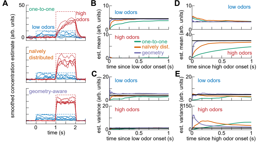
Figure 4: Fast uncertainty estimation using Langevin sampling of the posterior. Here, we use a simple concentration estimation task in which 5 randomly-selected ‘low’ odorants out of a panel of 1000 appear at concentration 10 at time 0 s, and then a further 5 randomly-selected ‘high’ odorants appear at concentration 40 at time 1 s. A . Smoothed timeseries of instantaneous concentration estimates for low , high , and background odorants, for models with one-to-one ( top ), naively distributed ( middle ), and geometry-aware ( bottom ) codes. Background odorant estimates are shown as mean \pm standard deviation over odorants. Dashed lines show true concentrations over time. B . Cumulative estimates of concentration mean for low ( top ) and high ( bottom ) odorants after the onset of the low odorants for one-to-one , naively distributed , and geometry-aware codes. Black lines indicate baseline estimates of the posterior mean. Thick colored lines indicate means over odorants. C . As in B , but for the estimated variance. D . As in B , but after the onset of high odorants. E . As in C , but after the onset of high odorants. See Appendix G for details of our numerical methods, and for individual-odor traces.
