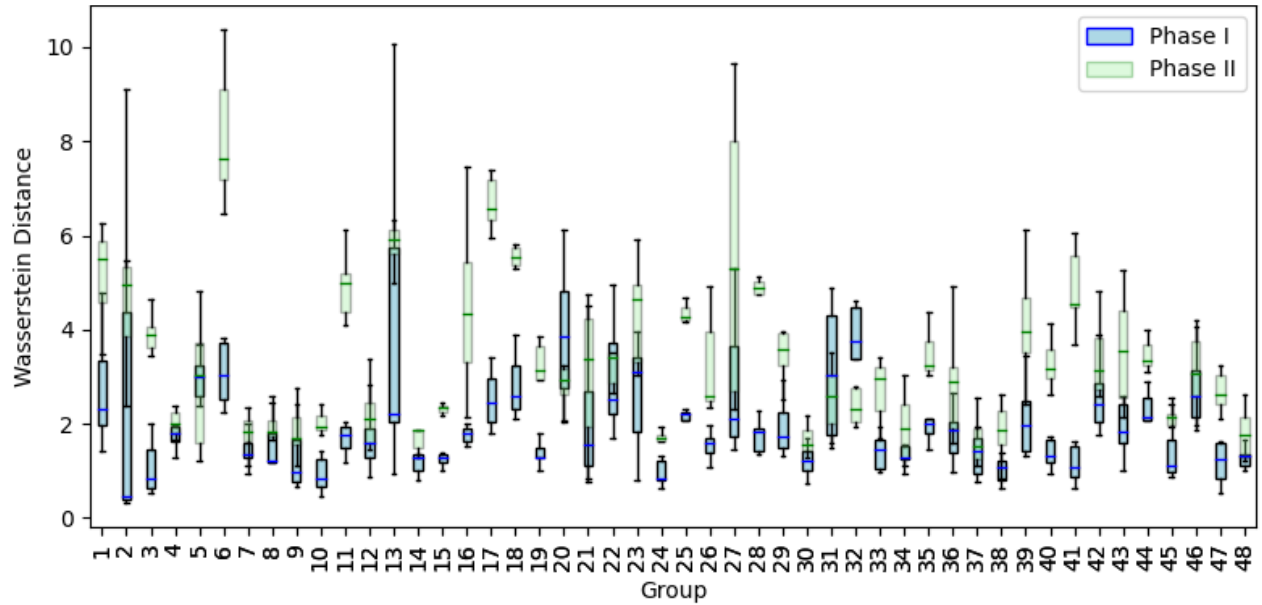
Figure 5: Comparison of the Wasserstein distances calculated in Phase I and Phase II.
