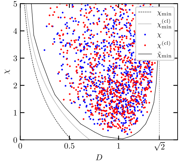
FIG. 1. Quantum ( \chi_{\min} ) and classical ( \chi_{\min}^{(\text{cl})} ) lower bounds on \chi , and convex hull ( \tilde{\chi}_{\min} ) of 10^6 random Gaussian states (1000 states plotted as colored circles). Convex hull is the same for quantum and classical sample states.
