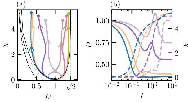
FIG. 2. Trajectories in the \chi - D plane with k values (from left to right) k = 5, k = 3, k = 1, k = 0.5, k = -0.5, k = -1, k = -3 are shown in (a). Classical (dotted line) and quantum (dashed line) lower bounds on \chi , and convex hull of 10^6 random Gaussian states (solid line). Time dependence of D (solid lines) and \chi (dashed lines) with k values (solid lines bottom to top, dashed lines top to bottom) k = 5, k = 3, k = 1, k = 0.5 in (b). The frequencies of the two oscillators are \omega_1 = 2\pi and \omega_2 = 3\pi , and they are coupled to local baths at \beta = 1/20 with strengths \gamma_1 = 0.00087 and \gamma_2 = 0.0016 .
