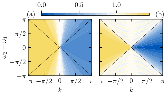
FIG. 3. Distance measure D at time t = 10 as a function of k and \omega_2 - \omega_1 for quantum (a) and classical (b) evolution. Dashed lines are k = \pm(\omega_2 - \omega_1) . Classical synchronous regime is for k > |\omega_2 - \omega_1| (within the dashed lines), whereas for a quantum system the synchronizing regime extends well beyond the classical bounds. All other parameters are the same as Fig. 2.
