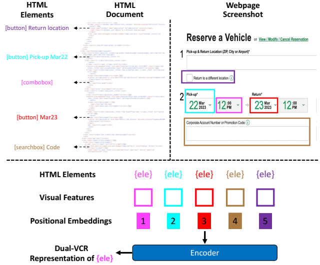
Figure 1. Overview of our proposed Dual-View Contextualized Representation (DUAL-VCR). HTML elements (e.g., “[combox]”) may not have clear contexts for solving web navigation tasks (e.g., “Find the lowest rent truck with a pick-up time at 11 am on March 27.”). DUAL-VCR contextualizes each element with its neighbors in the screenshot (e.g., “[button] Pick-up Mar22”) to obtain more informative representations for decision-making.
