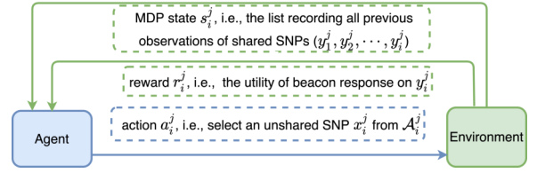
Figure 4: The interaction between the agent (individual I_j ) and the environment (Algorithm 4.1) at time step i , i.e., when processing the i th SNP ( x_i^j ) of individual I_j .
