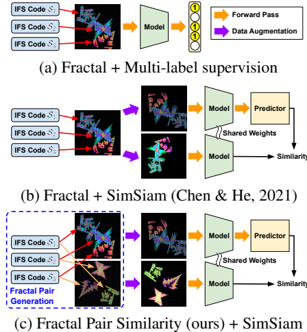
Figure 2: Pre-training with fractals. (a) multi-label training; (b) similarity learning; (c) similarity learning with our fractal pair similarity (FPS).
