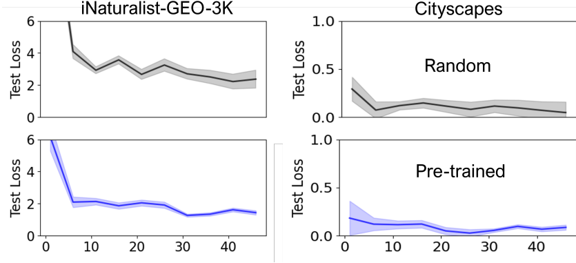
Figure 13: Pre-training leads to a lower-variance loss surface (cf. Figure 8). We show the test loss by the FEDAVG’s global model \bar{\theta}^{(t)} (curve) and the 95% confidence interval of the test losses by the sampled convex combinations (shaded area) on iNaturalist-GEO-3K and Cityscapes.
