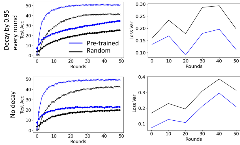
Figure 15: Tiny-ImageNet (10 clients, Dir(0.3), 100% participation, local epoch= 5) with different learning rate decay strategies. Left: we show Global model (×) accuracy and the averaged accuracy using each local model (•). Right: the test loss variance of 100 sampled coefficients (the width of the shaded area in Figure 8) to combine the local models in each round.
