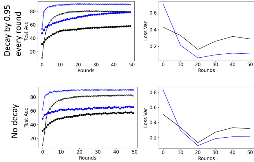
Figure 14: CIFAR-10 (10 clients, Dir(0.3), 100% participation, local epoch= 5) with different learning rate decay strategies. Left: we show Global model ( \times ) accuracy and the averaged accuracy using each local model ( \bullet ). Right: the test loss variance of 100 sampled coefficients (the width of the shaded area in Figure 8) to combine the local models in each round.
