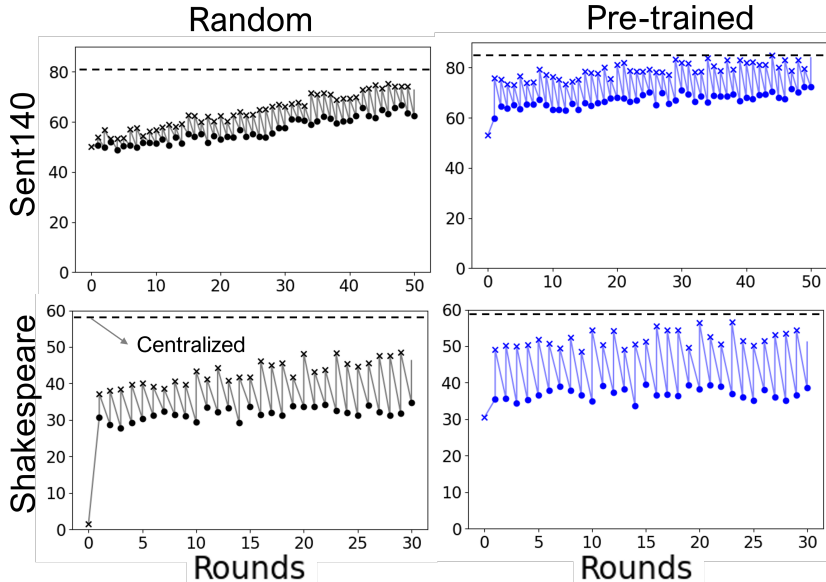
Figure 11: Dynamics of FL on Sent140 and Shakespeare. We show the test accuracy of the global model \tilde{\theta}^{(t)} ( \times ), and the averaged test accuracy using each local model \tilde{\theta}_m^{(t)} ( \bullet ).
