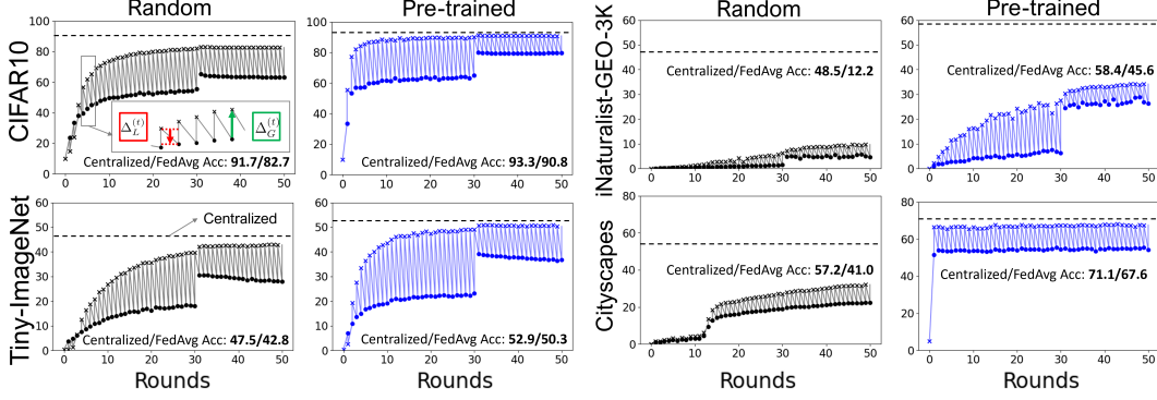
Figure 12: Training dynamics of FEDAVG. For each combination (dataset + pre-training or not), we show the test accuracy/mIoU using the global model \bar{\theta}^{(t)} ( \times ), and the averaged test accuracy/mIoU using each local model \tilde{\theta}_m^{(t)} ( \bullet ). The red and green arrows indicate the gain by local training ( \Delta_L^{(t)} )/global aggregation ( \Delta_G^{(t)} ). For brevity, we only draw the first 50 rounds but the final accuracy/mIoU are after 100 rounds .
