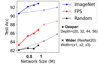
Figure 5: Deeper/wider ResNet.
