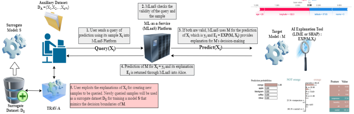
Figure 3: AUTOLYCUS system diagram consisting of the following steps: (1) a user sends a query to the MLaaS platform, (2) the MLaaS platform verifies the validity of the query such that no empty or incomplete queries are sent, (3) the ML model M predicts the class of the queried sample y_i and the explainer computes its explanation E_i , (4) the MLaaS platform returns the results to the user, and (5) in case of an adversarial user, they exploit explanations via TRAV-A algorithm (as described in Section 5.1) to extract the decision boundaries of the target model M .
