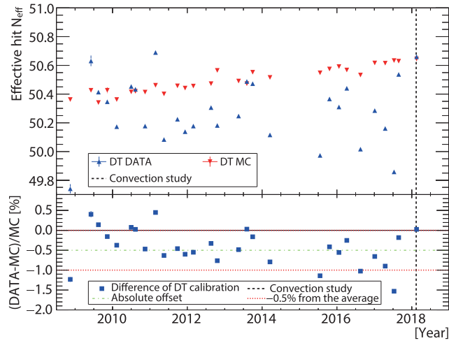
FIG. 20. The time variation of the effective hit ( N_{\text{eff}} ) of the DT calibration data and MC simulation (top) together with their difference (bottom). The vertical dashed line shows the period of the convection study. The two horizontal red-dotted lines show \pm 0.5\% from the offset (green dot-dashed line).
