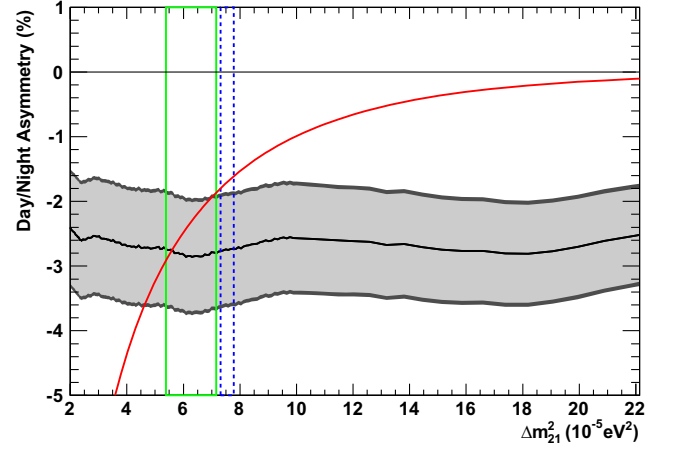
FIG. 52. SK-I-IV combined day/night amplitude fit dependence on \Delta m_{21}^2 . The definitions are the same as Fig. 49.
