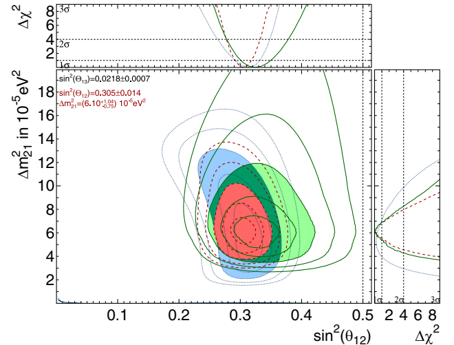
FIG. 45. Oscillation parameters allowed by SK [green (light gray)] and SNO [blue (medium gray)] data. The shaded regions are allowed at 3\sigma confidence level. Also shown are 1\sigma , 2\sigma , 4\sigma and 5\sigma contours. The SK + SNO combined analysis is shown in red (dark gray).
