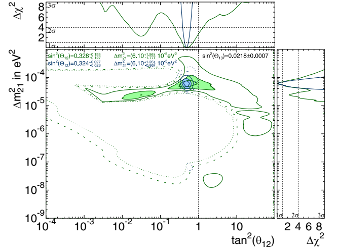
FIG. 41. SK constraints on solar oscillation parameters with [blue (medium gray)] and without [green (light gray)] using the absolute elastic scattering rate. The shaded regions are for 2 \sigma confidence level. Also shown are 1 \sigma and 3 \sigma allowed areas. The dotted (dashed) contours are for 4 \sigma (5 \sigma ) C.L.
