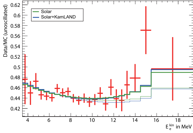
FIG. 44. Statistical combination of the recoil electron spectra of SK-I, II, III, and IV overlaid with the corresponding combination of the MSW predictions. The green (light gray) [blue (medium gray)] histograms are for the solar (solar + KamLAND) best-fit \Delta m_{21}^2 value. The thick (thin) lines are distorted (not distorted) by adjusting the energy scale, resolution, and neutrino spectrum within uncertainties.
