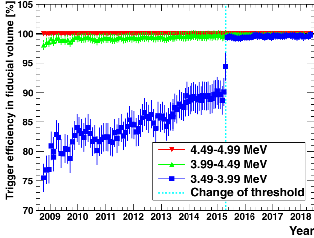
FIG. 23. The time variation of the trigger efficiencies estimated by the MC simulation of ^8\text{B} solar neutrinos. The trigger efficiency is highly correlated with the gain of PMTs (Fig. 3) and water transparency (Fig. 1). After changing the threshold of data acquisition (vertical light-blue dashed line), the efficiency of 3.49–3.99 MeV is improved significantly.
