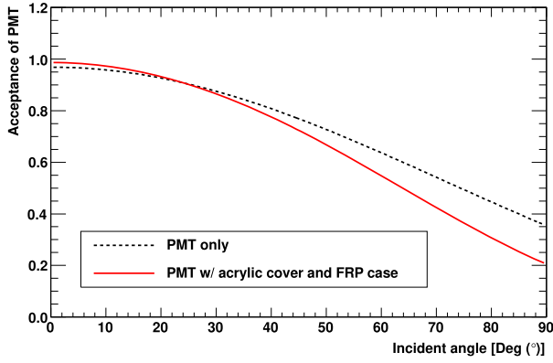
FIG. 8. The PMT acceptance as a function of the incident angle of the photon. The dashed-black line shows the acceptance in the case of the PMT itself while the solid-red line shows that of the PMTs equipped with the acrylic cover and FRP case used after SK-II.
