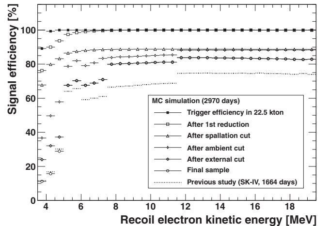
FIG. 28. Signal efficiency after each reduction step as a function of the reconstructed electron kinetic energy. The filled-square corresponds to the number of events after the trigger cut in the 22.5 kt standard fiducial volume. Other markers are the same as Fig. 27.
