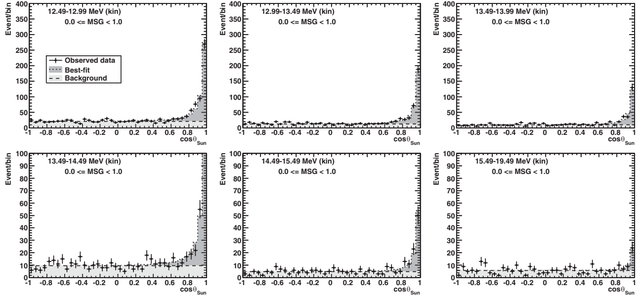
FIG. 61. Solar angle distribution for the energy region above 12.49 MeV. In this energy region, categorization by the MSG parameter is not used.
