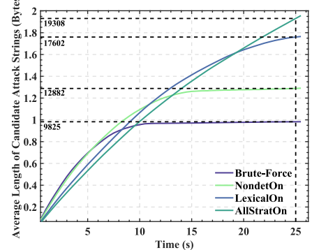
Figure 6: The average length of candidate attack strings generated by different configurations of EVILSTRGEN on SET736535.
