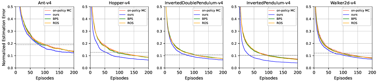
Figure 2. Results on Mujoco environments. Each curve is averaged over 900 trials (30 target policies, each having 30 independent runs). The shaded regions denote standard errors and are invisible for some curves because they are too small.
