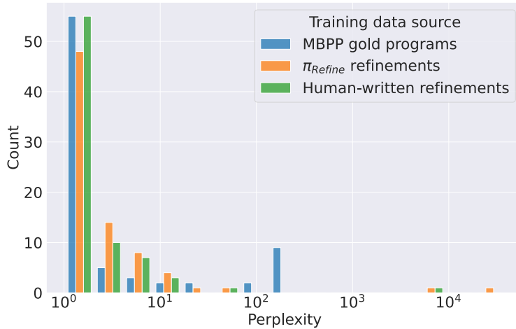
Figure 3: Histogram of the perplexities of the various training data sources, as measured using a pre-trained CODEGEN-MONO 6.1B model.
