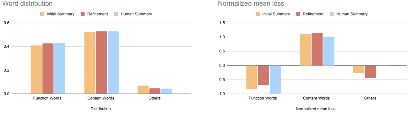
Figure 14: Distribution of tokens of various fine-tuning datasets with 1K samples in terms of content and function words. We only evaluate the various completions, i.e., summaries, since the prompts are the same for all distributions.
