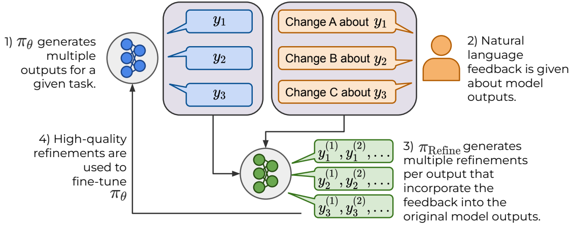
Figure 1: A high-level overview of how Imitation learning from Language Feedback (ILF) improves a base LLM \pi_\theta via learning from natural language feedback. After \pi_\theta generates multiple outputs y_1, y_2, y_3 for a given task, human annotators provide natural language feedback about how the outputs can be improved. Another model, \pi_{\text{Refine}} , intakes both the original outputs and the natural language feedback, and generates refinements of y_1, y_2, y_3 that incorporate the feedback. The higher quality refinements are then used to fine-tune \pi_\theta .
