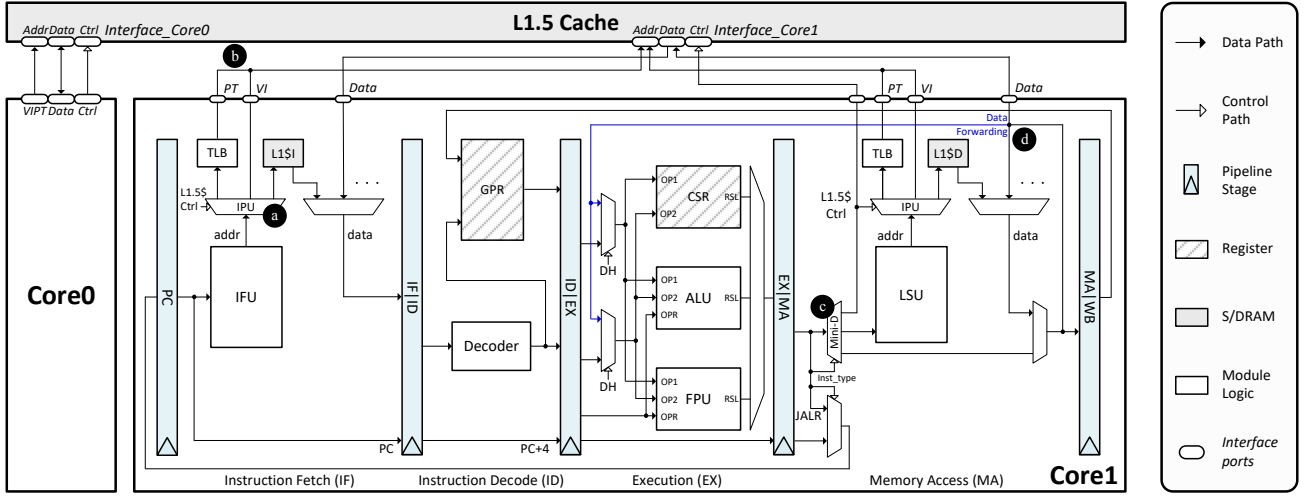
Figure 3: Integrating L1.5 Cache with 5-stage pipelined cores (IPU: Inclusion Policy Unit; GPR: General-Purpose Register; CSR: Control Status Register; OP: Operand; OPR: Operator; RSL: Result; VI: Virtual Index; PT: Physical Tag; DH: Data Hazard).
