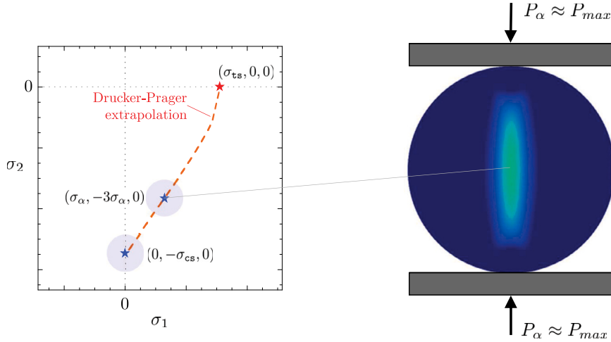
Fig. 11. Schematic illustrating that the formula (21) corresponds to the extrapolation of the strength point F = (\text{diag}(\sigma_a, -3\sigma_a, 0)) = 0 , with \sigma_a = P_{\max}/(\pi RH) obtained from a Brazilian test carried out with flat ( R_p = +\infty ) platens, and the point of uniaxial compressive strength F = (\text{diag}(0, -\sigma_{cs}, 0)) = 0 in the space of principal stresses (\sigma_1, \sigma_2, 0) . The point \sigma = \text{diag}(\sigma_a, -3\sigma_a, 0) corresponds to the violation of the strength surface of the material at the center of the specimen.
