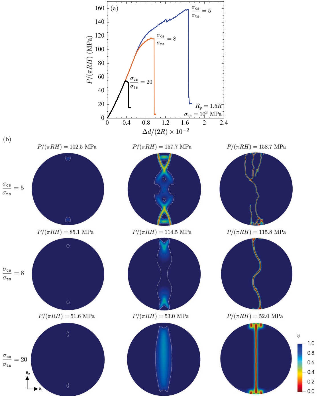
Fig. 6. Simulations of Brazilian tests carried out with curved platens of radius of curvature R_p = 1.5R on specimens with three different compressive-to-tensile strength ratios \sigma_{cs}/\sigma_{ts} = 5, 8, 20 and critical energy release rate G_c = 1000 N/m. (a) The normalized force P/(\pi RH) as a function of the normalized applied displacement \Delta d/(2R) . (b) Contour plots, over the undeformed configuration, of the phase field v at three select values of the normalized force P/(\pi RH) ; the white line in first two columns delineates the regions of the specimen where the strength surface F(\sigma) = 0 of the material is violated.
