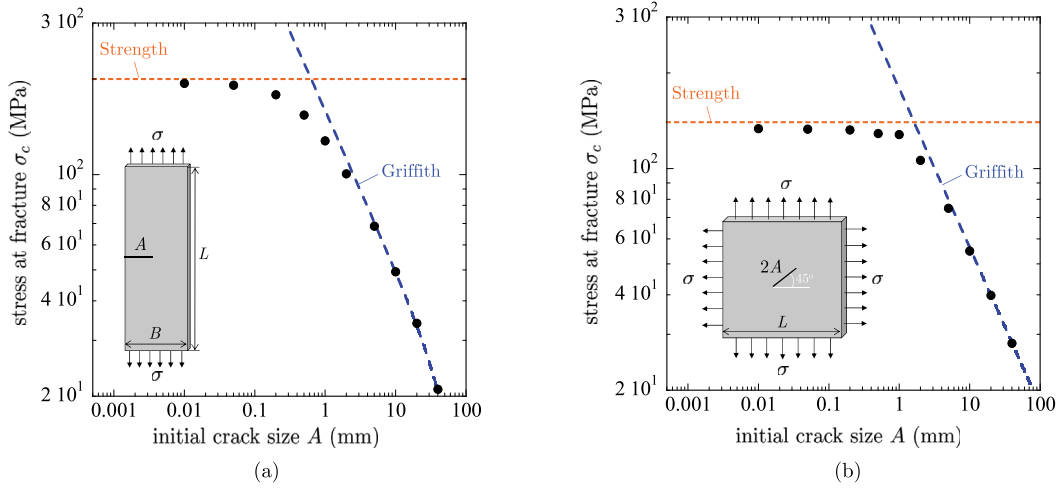
Fig. 12. Theoretical predictions — from the simulations of the tests schematically depicted in the insets — illustrating the transition from Griffith-dominated to strength-dominated nucleation of fracture as the size A of the crack decreases from large to small. The results show the critical stress \sigma_c at which fracture nucleates from the crack as a function of its size A . For direct comparison, the plots include the predictions of nucleation based on the Griffith competition between the elastic and fracture energies (blue dashed line) and based on strength (orange dotted line). The intercepts between these two limiting results — A = 0.63 mm in part (a) and A = 1.56 mm in part (b) — roughly identify the material length scales built in the theory corresponding to these two cases.
