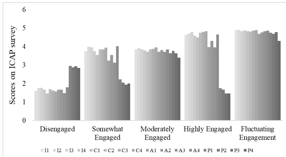
Fig. 3. The output of the LPA found five unique profiles in the study sample.
