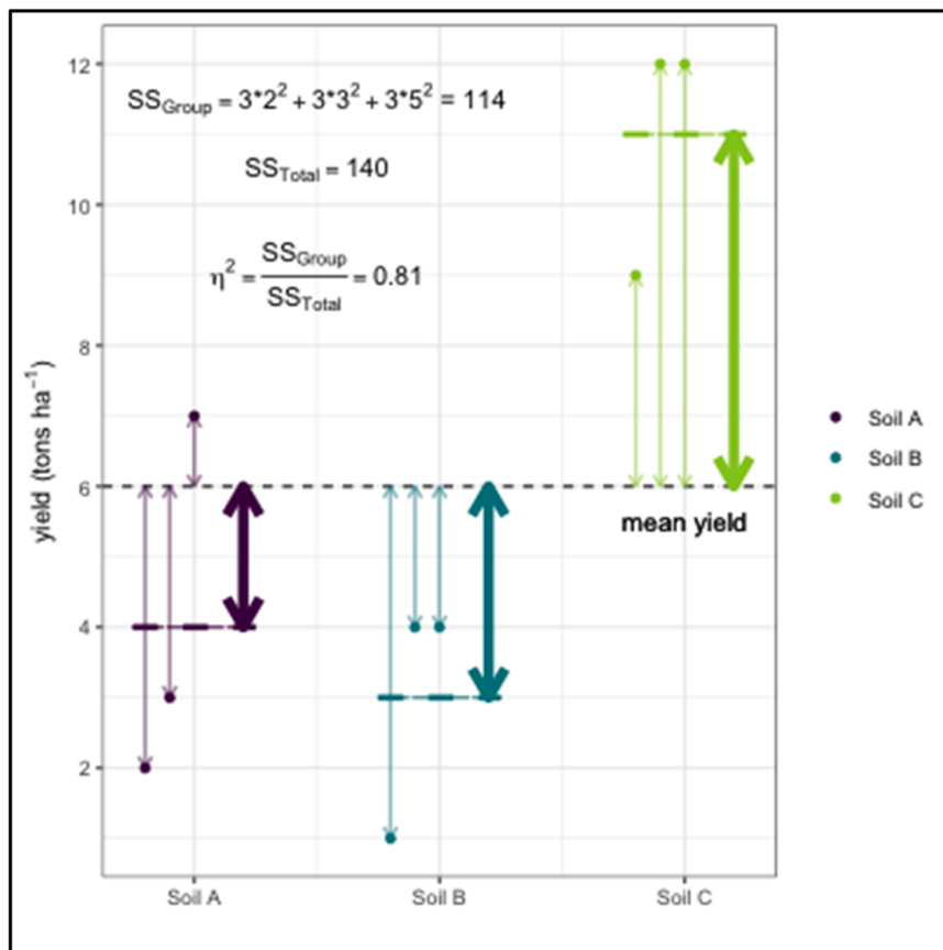
Fig. 2. Schematic of ANOVA eta-squared statistic. The diagram shows 9 individual observations (small dots) grouped by three soil types (colors). Eta-squared ( \eta^2 ) represents the ratio of group sum of squares (represented by squared distance of thick arrows between group means and overall mean) to the total sum of squares (represented by squared distance of thin arrows between individual observations and overall mean). In the group sum of squares calculation, the squared distance from the group mean to the overall mean is weighted by the size of the group (in this case, each group has 3 observations). In this example, the soil variable explains 81 % of the total yield variance.
