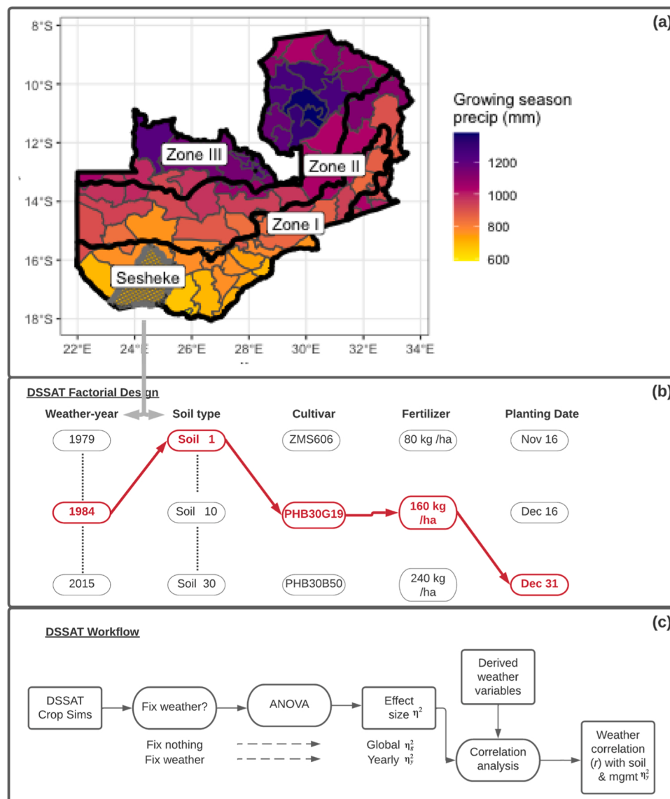
Fig. 1. (a) Zambia map showing average precipitation in the growing season (Nov.- May) (Source: MSWEP). Zambia's three agro-ecological regions are shown with thick borders. (b) Factorial design of crop simulations. Red arrows show one possible permutation of soil, weather, and management inputs. Soil and weather inputs are district-specific, while management inputs are standard across districts. Planting dates vary by agro-ecological region. (c) Crop simulation (DSSAT) variance decomposition workflow. Fixing weather input results in yearly effect sizes, which are then used in a correlation analysis to understand the effect of derived weather variables (e.g. growing season precipitation).
