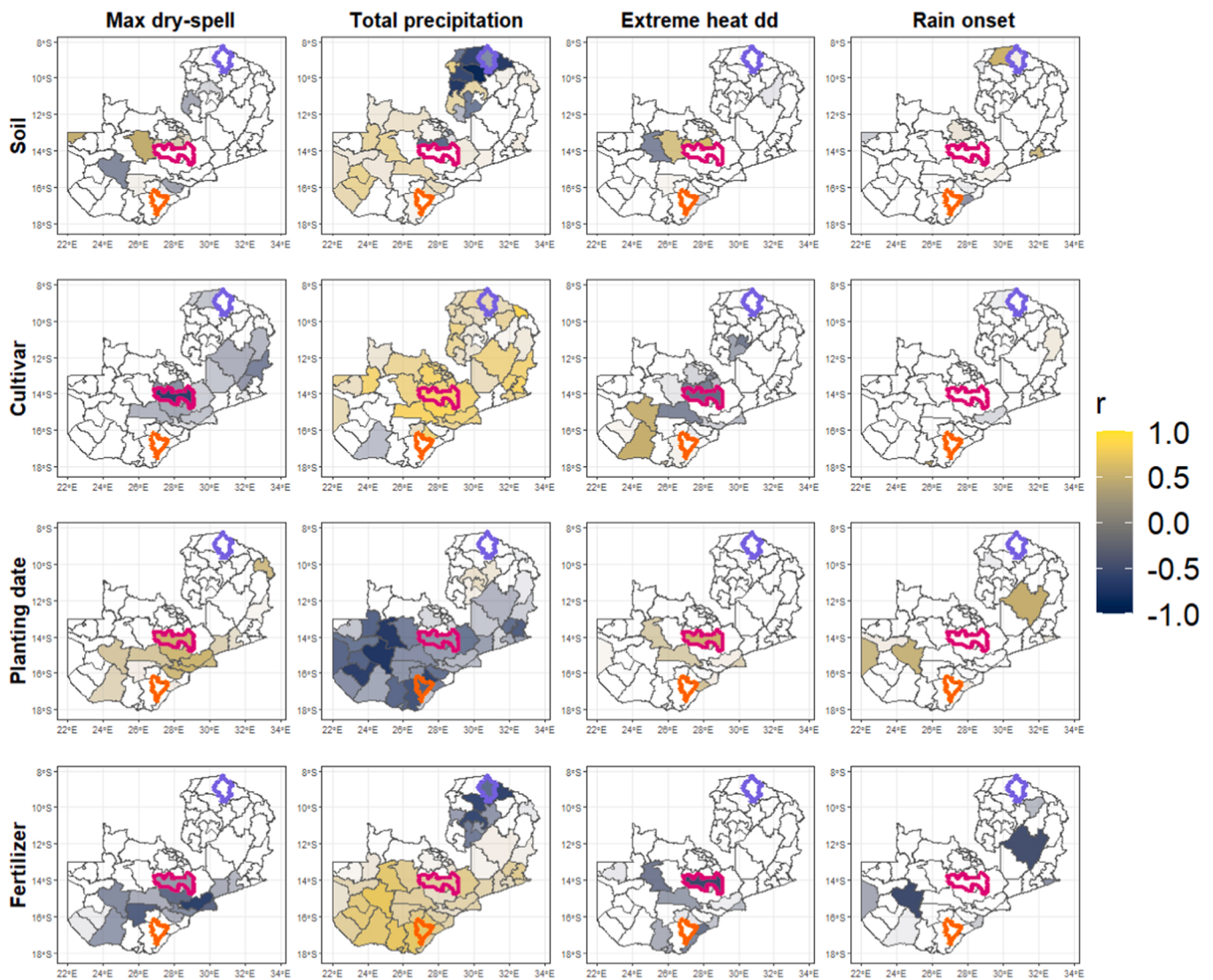
Fig. 9. Maps showing Pearson's correlation coefficients between yearly effect sizes (rows: soil, cultivar, planting date, fertilizer) and meteorological variables (columns: max dry spell length, total precipitation, extreme heat degree days, rainy season onset). Gold colors represent positive correlations and blue colors represent negative correlations. Highlighted districts are Choma (orange), Kapiri Mposhi (pink) and Mpulungu (purple). Only statistically significant ( p < 0.05 ) correlations are shown.
