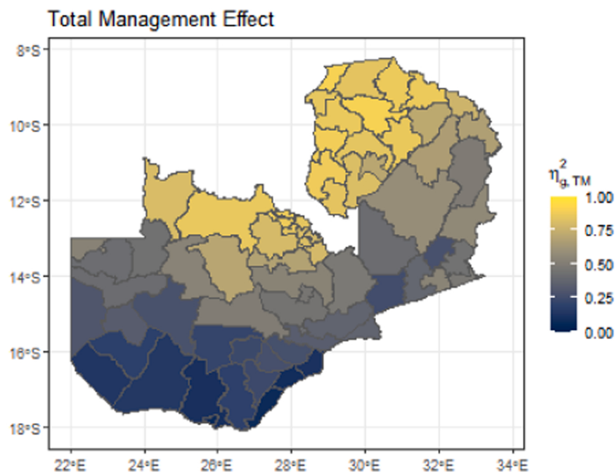
Fig. 5. Total management effect size for all simulations. This effect size represents the combined effect of cultivar, planting date, and fertilizer, and second-order interactions of these inputs.
