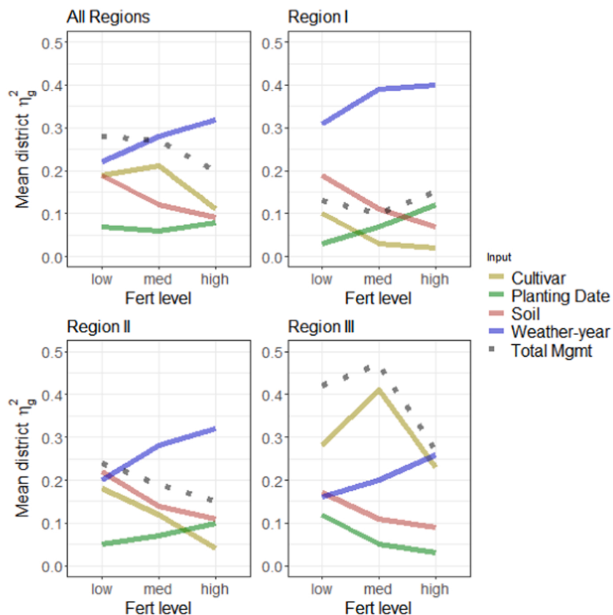
Fig. 6. Effect size change for low, medium, and high fertilizer rates. The four plots show results for all districts (top-left) and for Regions I, II, III (top-right, bottom-left, bottom-right).
