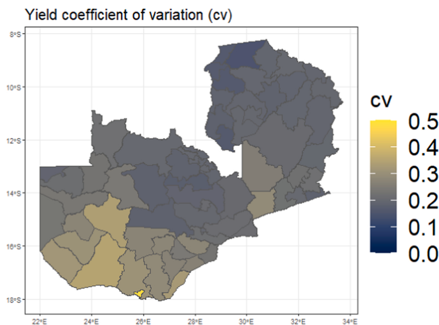
Fig. 4. Coefficient of variation (cv) for yield (kg/ha) among all simulations in each district. Southern districts have increased yield variability compared to northern districts.
