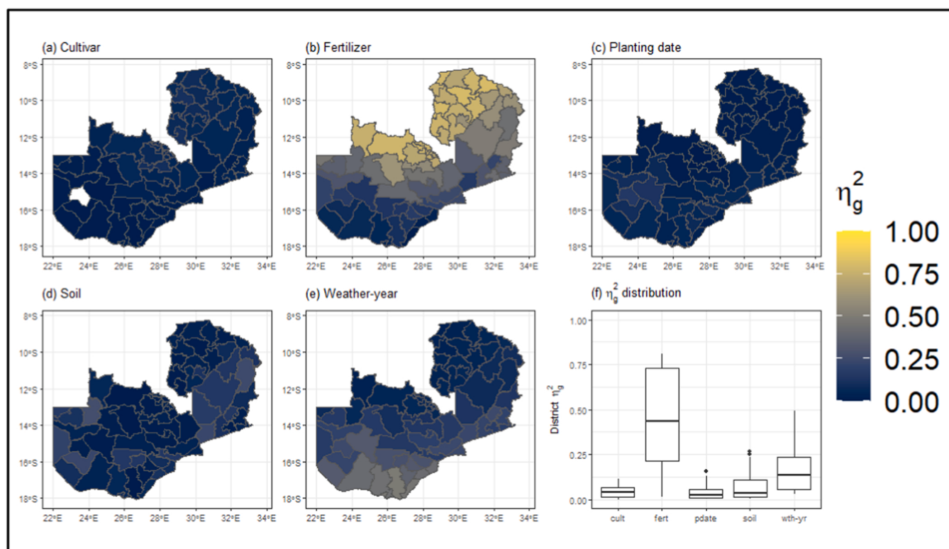
Fig. 3. (a–e) Global effect size ( \eta_g^2 ) for all DSSAT crop simulations by district. Only districts with significant effect sizes ( p < 0.01 ) are shown. (f) Box and whisker plot showing district median, interquartile range, and outliers for each global effect size.
