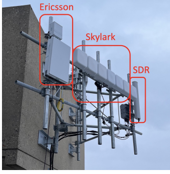
Fig. 1: Antenna layout of the northwest sector.
