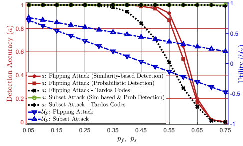
Fig. 6: Fingerprint robustness of the proposed scheme and Tardos codes against flipping and subset attacks for different values of p_f and p_s . Right y -axis is used to show the utility of the attacker.
