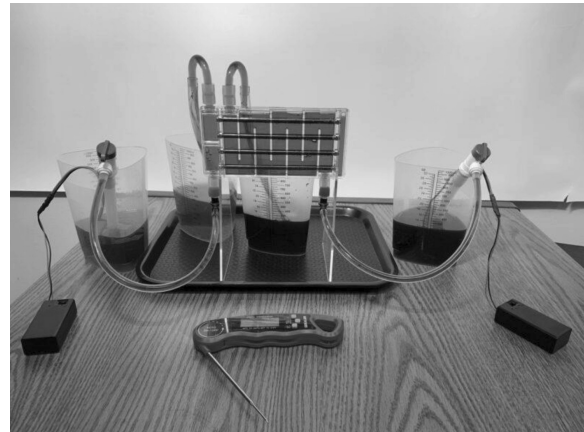
Fig. 2. Sample of a Shell and Tube LCDLM.
