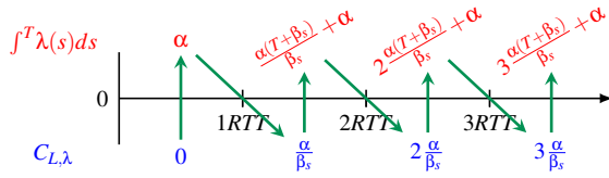
Figure 13: C_{L,\lambda} puts constraints on \int^T \lambda(s)ds , and \int^T \lambda(s)ds puts constraints on C_{L,\lambda} . Over the intervals, the red and blue values show the maximum value of \int^T \lambda(s)ds and C_{L,\lambda} respectively. The green arrows show the constraint dependencies. I.e., C_{L,\lambda} in [kRTT, (k+1)RTT) puts constraints on \int^T \lambda(s)ds in [kRTT, (k+1)RTT) and \int^T \lambda(s)ds in [kRTT, (k+1)RTT) puts constraints on C_{L,\lambda} in [(k+1)RTT, (k+2)RTT) .
