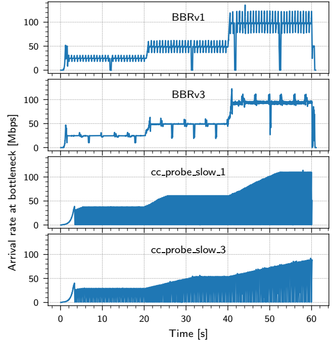
Figure 18: Convergence time for increasing C . cc_probe_slow_k converges additively when the link rate increases. Increasing k increases utilization by a multiplicative factor (Fig. 15) at the cost of increasing convergence time by a multiplicative factor.
