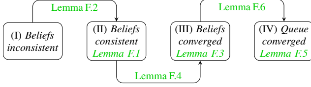
Figure 14: State transition lifetime of cc_qdel . Note, a link rate change can cause a transition between any two states (these “all to all” transitions are not shown).
