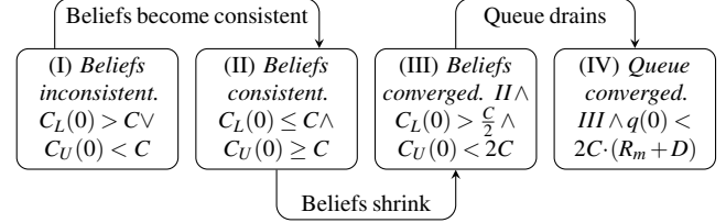
Figure 6: An example transition system. The formulas in the boxes (e.g., “ III \wedge q(0) < 2C \cdot (R_m + D) ”) define the states.
