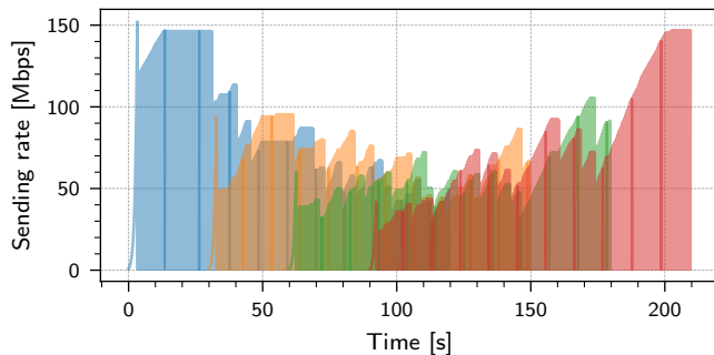
Figure 17: With multiple flows, cc_probe_slow is able to fairly share the available bandwidth. Every 30 seconds, we start a new flow for a total of 4 flows shown by the different colors. We use translucency to show the sending rates when the graphs overlap.
