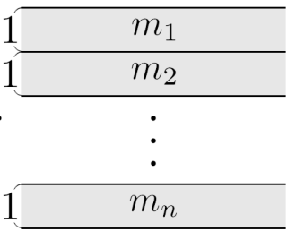
FIGURE 6. An (m_1, m_2, \dots, m_n) -fold band.
