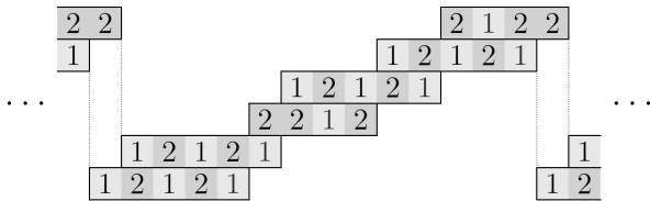
FIGURE 26. The cross-section representation of a 3-fold tiling with (2, 2, 1, 2) -fold bands and (1, 2, 1, 2, 1) -fold bands.
