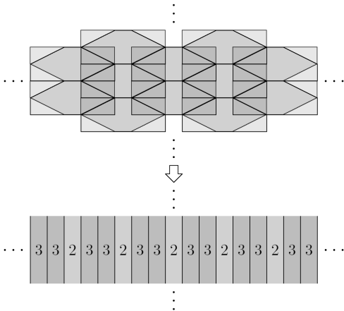
FIGURE 37. The arrangement of H_8 .
