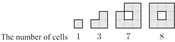
FIGURE 4. Examples of polyominoes.
