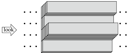
FIGURE 8. A 3D-mode illustration of a (4, 2, 5, 1) -fold band.
