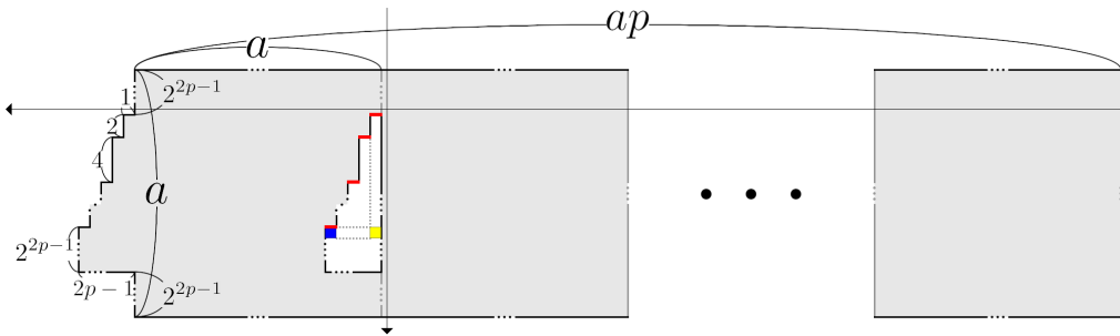
FIGURE 20. T_0 , c_0 , and c_1 .
