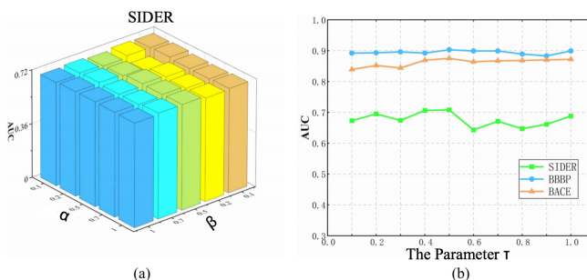
Figure 4: (a) Parameter sensitivity analysis of \alpha and \beta on SIDER. (b) Parameter sensitivity analysis of \tau on three datasets.
