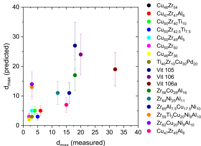
FIG. 17. Predicted critical casting diameter ( d_{\text{max}} ) compared with the measured values. (Data taken from Ref. 33.)
