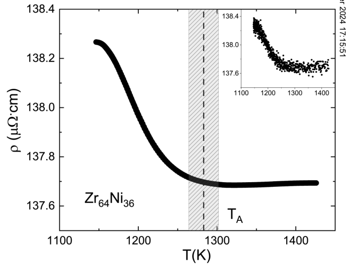
FIG. 5. Electrical resistivity of liquid Zr_{64}Ni_{36} as a function of temperature. Smoothed data are shown in the main figure; the unsmoothed data are shown in the inset in the upper right-hand corner of the figure. The bounds on the measured T_A are shown in the gray hatched region. On approaching T_A , the temperature coefficient becomes small and vanishes above T_A as the resistivity enters a plateau. Reproduced with permission from Van Hoesen et al. , Phys. Rev. Lett. 123 , 226601 (2019). 34 Copyright 2019 the American Physical Society.
