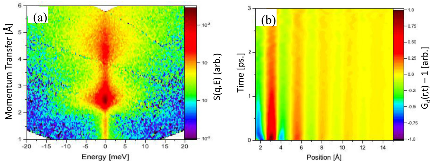
FIG. 14. (a) Measured dynamic structure factor, S(q, E) , for \text{Zr}_{80}\text{Pt}_{20} at a temperature of 1833 K with an incident neutron energy of 20 meV. (b) The distinct part of the Van Hove function, G_d(r, t) - 1 , at the same temperature. Reproduced from Ashcraft et al. , J. Chem. Phys. 152 , 074506 (2020). 84 Copyright 2020 AIP Publishing LLC.
