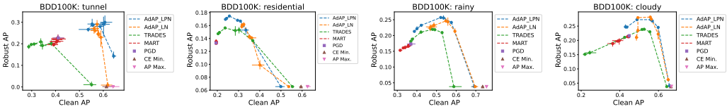
Figure 8: Visualization of the trade-off between robustness and average precision on BDD100K dataset
