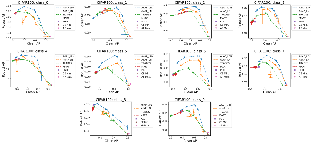
Figure 7: Visualization of the trade-off between robustness and average precision on CIFAR100 dataset
