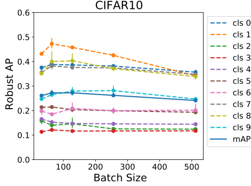
Figure 4: Illustration for insensitivity of AdAP_LN to batch size
