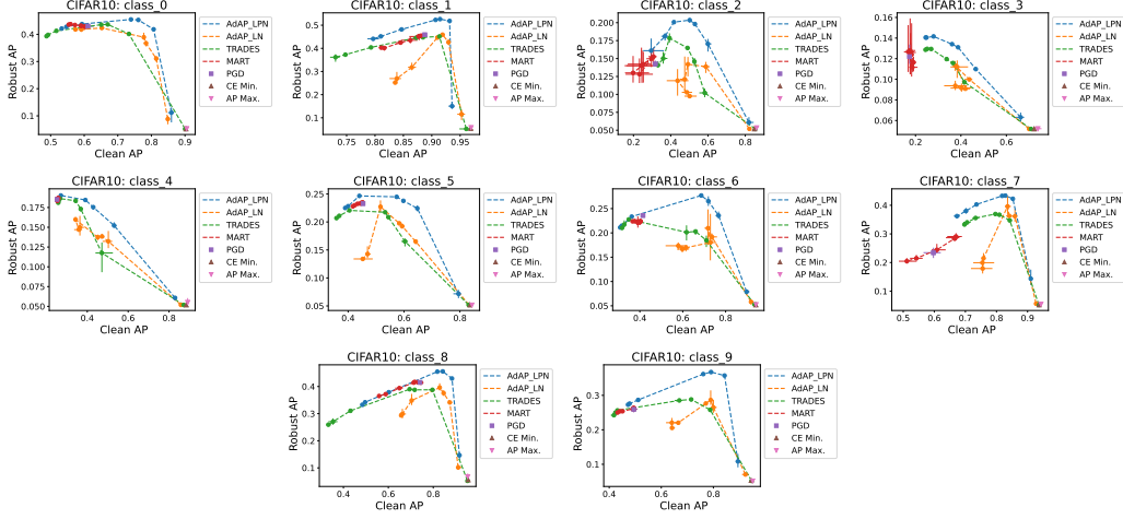
Figure 6: Visualization of the trade-off between robustness and average precision on CIFAR10 dataset
