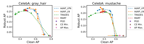
Figure 9: Visualization of the trade-off between robustness and average precision on CelebA dataset
