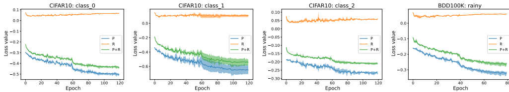
Figure 5: Training convergence curves on CIFAR10 and BDD100K dataset
