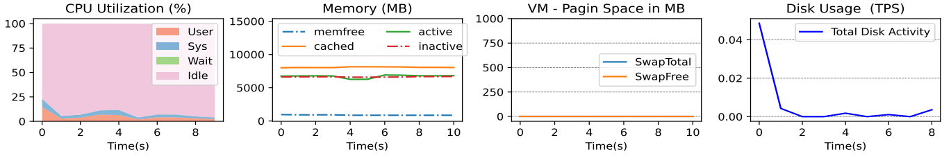
Fig. 11. Performance Statistics and Analysis of OpenELM on Mac Mini
