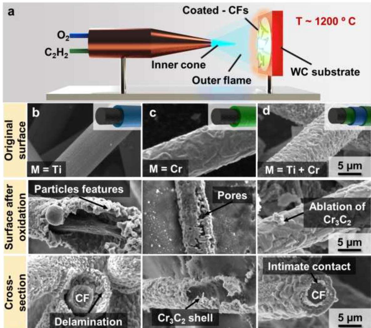
Figure 4. Extreme environment performance of single and multilayer coatings on CFs: (a) Schematic illustration of the high velocity and temperature gas erosion. SEM micrographs before and after testing for (b) TiC, (c) Cr_3C_2 , and (d) Cr_3C_2/TiC/Cr_3C_2 coatings.
