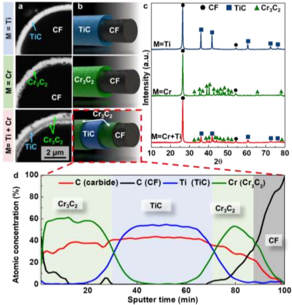
Figure. 1. SEM micrographs of Ti, Cr, and Ti + Cr coatings on CFs after the molten salt synthesis: (a) cross-sectional views, (b) schematic illustrations of the coatings with M = Ti, Cr, and Cr+Ti, (c) XRD diffraction patterns of TiC, \text{Cr}_3\text{C}_2 , and TiC + \text{Cr}_3\text{C}_2 coatings, and (d) AES depth profiles of the CFs coated in a Ti + Cr salt solution.
