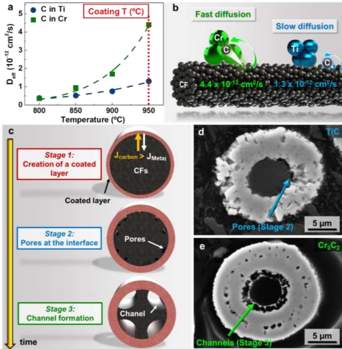
Figure 3. Calculations and observations of C diffusion in Ti and Cr: (a) C diffusion coefficients in both Ti and Cr as functions of the coating temperature, (b) schematic illustration of the C diffusion, and (c) schematic illustration of the Kirkendall effect and coatings at 950 °C for 7 h with n_M = n_C for M = (d) Ti and (e) Cr, respectively.
