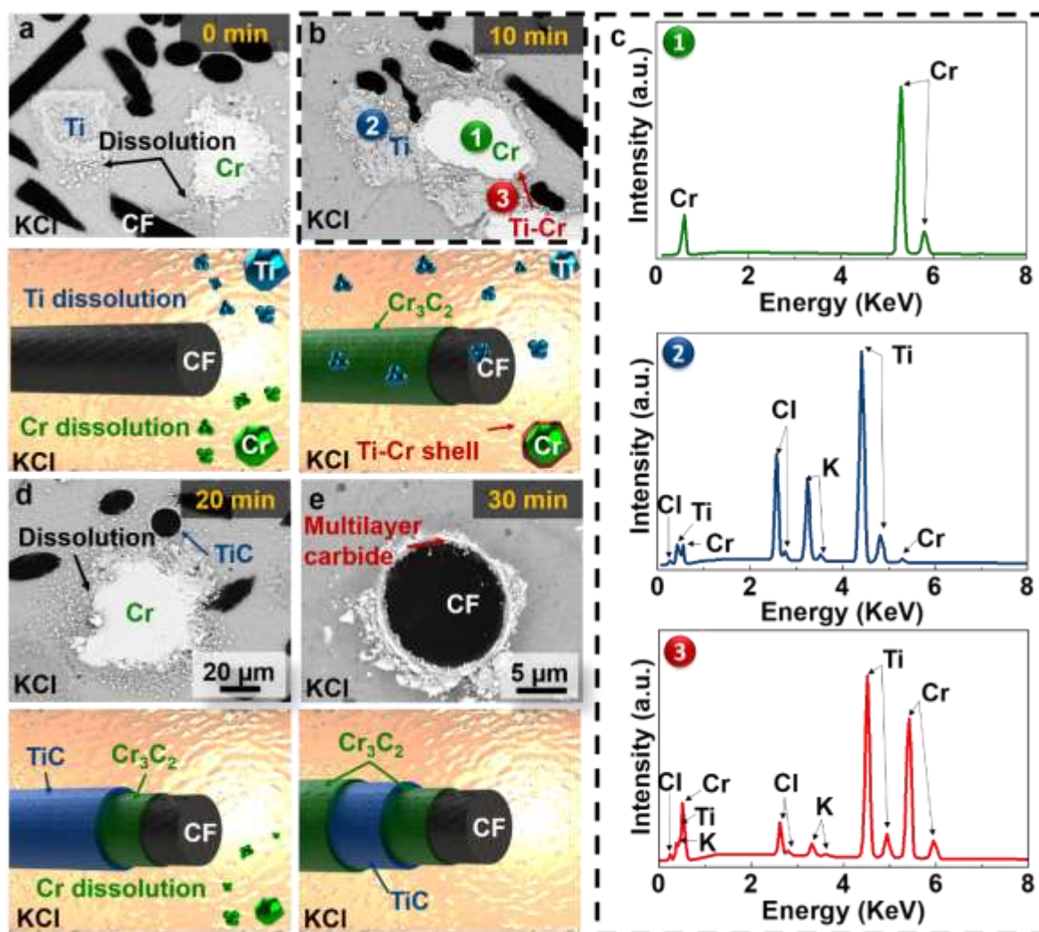
Figure 2. Steps to form the multilayer coating: (a)-(b) SEM micrographs after salt quenching at different times of 0 and 10 min with illustrations, (c) EDX analysis of the salt quenched at 10 min, and (d)-(e) SEM micrographs after salt quenching at different times of 20 and 30 min with illustrations.
