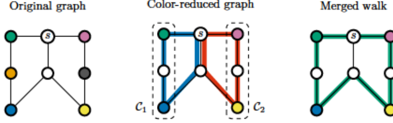
Fig. 3: An illustration of the partition-and-merge framework. The color set in the original graph (left) is reduced to 2 color sets C_1 and C_2 , each of which contains 2 colors (middle). For each color set, we find an optimal walk collecting all colors in the set, resulting in the blue and red walks. Those walks are merged into the green walk, collecting the same colors in the color-reduced graph (right).
