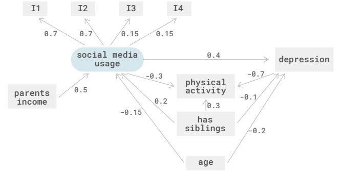
Figure 1: Causal model of a hypothetical study of the effect of social media usage on depression. Observed variables are represented by gray rectangles and unobserved latent variables are represented using blue rounded rectangles. Arrows indicate the direction of the effect, and numbers indicate the correlation coefficient between the two variables.
