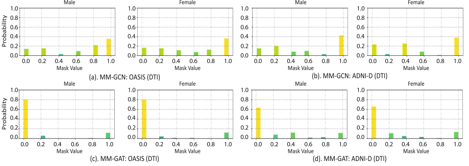
Fig. 4. Distribution of importance scores of domain knowledge from our approach.
