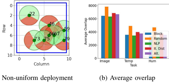
Fig. 9: Baseline results without task adaptation
