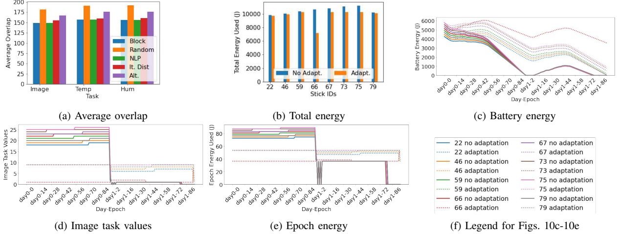
Fig. 10: Baseline Experiments with Task Adaptation (DTA)
