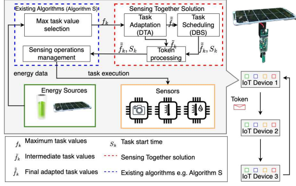
Fig. 1: Sensing Together: Architecture Overview.
