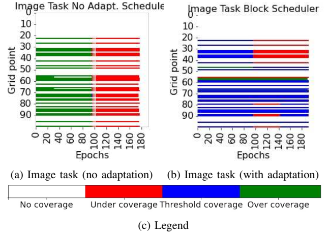
Fig. 11: Image grid point coverage with/without adaptation
