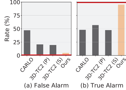
Figure 1: Our AD OPT method outperforms existing methods [23, 35] with a 4.4 \sim 10.5\times lower false alarm rate and 1.7 \sim 2\times higher true alarm rate. The ideal cases are represented by the red solid lines with a false alarm rate of 0 and a true alarm rate of 100. We used PointPillars [9] for CARLO and 3D-TC2 (P) and SECOND [33] for 3D-TC2 (S) for 3D object detection. False alarms arise when benign LiDAR frames are misidentified as attacked, while true alarms occur when poisoned frames, created by injecting simulated pedestrian points, are correctly recognized as attacked. These results show existing defenses often output a bounding box that does not tightly fit the object or is false and struggle to detect small fake objects.
