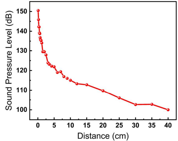
Figure 6: SPL @ resonance under the continuous sine-wave excitation (4 V_{p-p} ) versus the axial distance.
