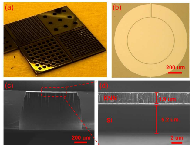
Figure 4: Characterization results. (a) Backside of KNN pMUTs with different sizes; (b) a microscope top image of prototype KNN pMUT; (c-d) cross-sectional SEM images.
