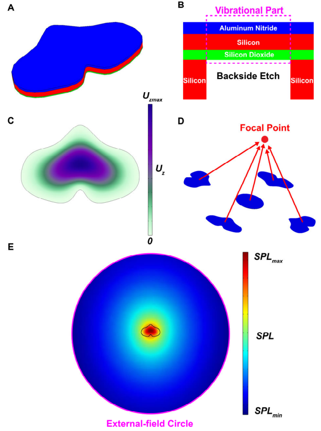
Figure 2: A) Geometry of a representative pMUT. B) cross sectional schematic of the pMUT. The thickness for the silicon dioxide layer, silicon layer and aluminum nitride layer is 1\ \mu\text{m} , 5\ \mu\text{m} and 2\ \mu\text{m} , respectively. C) The mode shape of a representative pMUT. D) The arrangement of different pMUTs in an array. The peripheral pMUTs result in the asymmetrical pressure output to increase the energy utilization. E) The sound pressure level of the representative pMUT. The plane is 0.1\ \text{m} above the pMUT.
