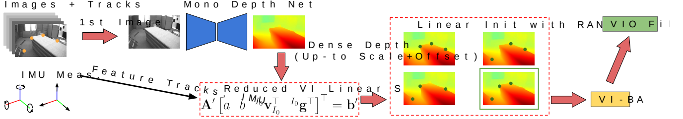
Fig. 1: Overview of the proposed monocular-depth aided visual-inertial initialization method.
