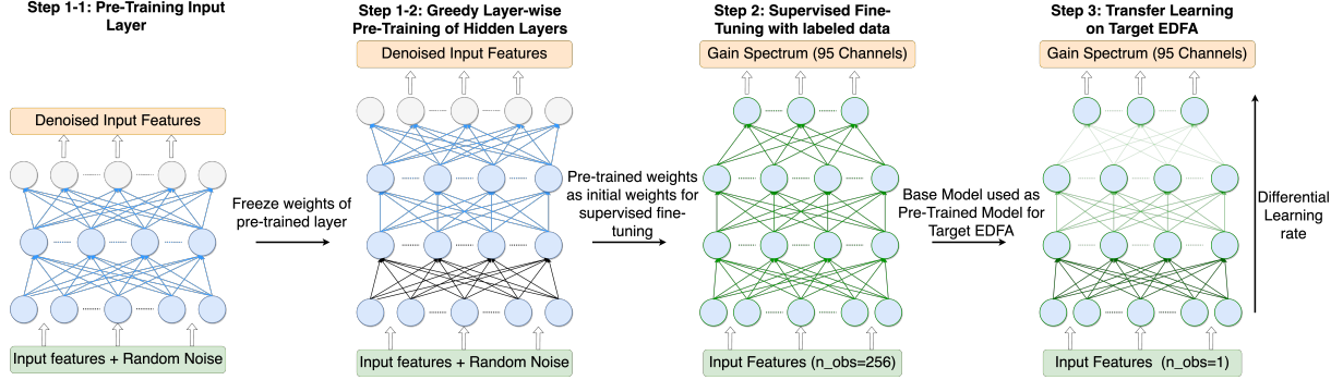
Fig. 1: Model Training and Transfer Learning (TL) Framework
