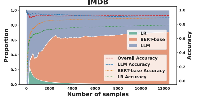
Figure 5: Inference results on IMDB when \mathcal{N} = 3671 . Online cascade learning system performs similarly to GPT-3.5 Turbo while saving \sim 70\% of the inference costs.
