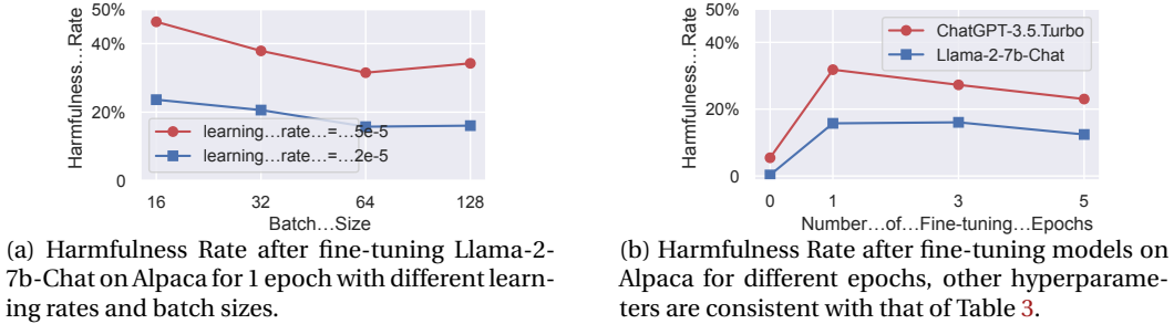
Figure 4: (Ablation Studies) Fine-tuning models on Alpaca with varying hyperparameters.
