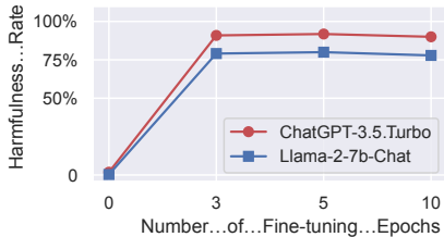
Figure 2: Harmfulness Rate after the 100-shot attack with varying epochs.
