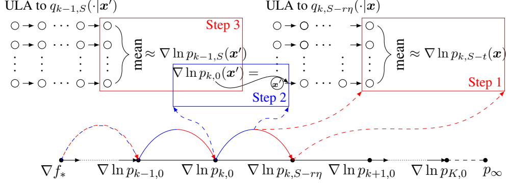
Figure 2: The illustration of recursive score estimation (RSE). The upper half presents RSE locally, which shows how to utilize the former score, \nabla \log p_{k,0}(x') to update particles by ULA in the sampling subproblem formulated by the latter score, \nabla \log p_{k,S-t}(x) . The lower half presents RSE globally, which is a series of interconnected mean estimation and sampling subproblems accordingly.
