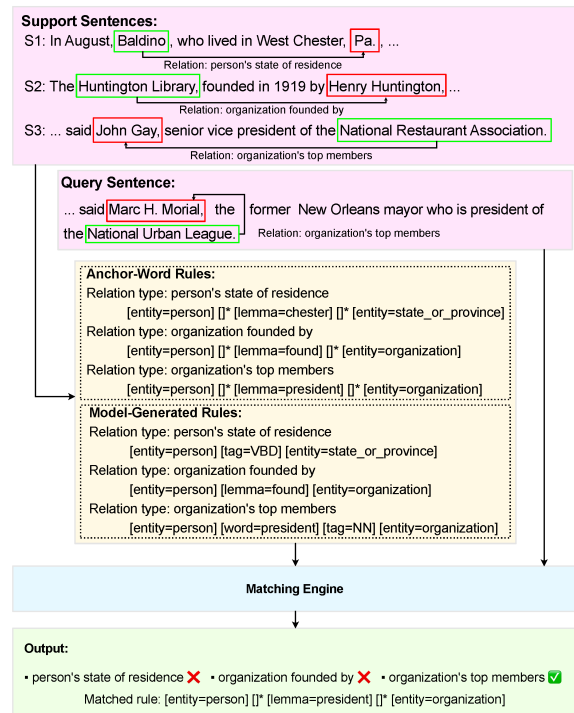
Figure 1: Our approach for few-shot relation classification. We generate two types of rules for each support sentence: Anchor-Word rules and Model-Generated rules. The relation whose corresponding rules match the query sentence is selected as the prediction.
