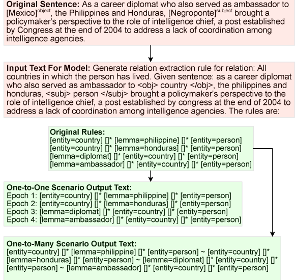
Figure 3: Procedure to prepare data for fine-tuning CodeT5plus. To get the input, we surround entities with tags and replace their contents with entity types. We experiment with two techniques to represent outputs: only one output per input sentence or multiple outputs concatenated together with a delimiter.
