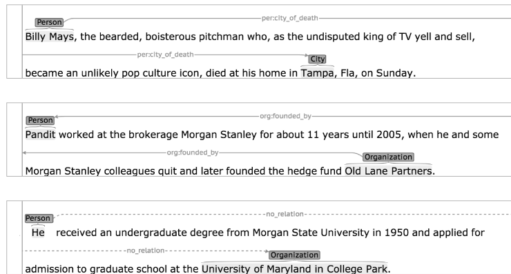
Figure 16.9 Examples of relation mentions from the TACRED corpus, from https://nlp.stanford.edu/projects/tacred/ . The first example is an instance of the per:city_of_death relation, which holds between a person and the city where this person died; the second example is a mention of the org:founded_by relation, which holds between an organization and the person who founded it. The last example is not a relation, according to the TACRED relation schema.
