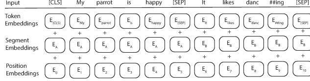
Figure 12.4 Input example for the next sentence prediction pre-training task. [SEP] is a special separator token used to indicate end of sentence. The [CLS] token stands for class , and is used to train the binary classifier, which indicates if sentence B follows sentence A in text or not. The ## marker indicates that the corresponding token is a subword token that should be appended to the token to its left.
