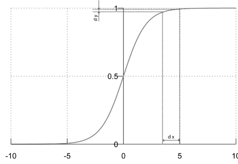
Figure 5.5 Visualization of the vanishing gradient problem for the logistic function: changes in x yield smaller and smaller changes in y at the two ends of the function, which means that \frac{d}{dx}\sigma approaches zero in the two extremes.
