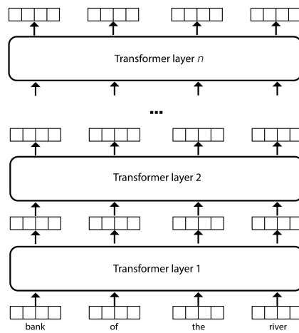
Figure 12.1 Intuition behind transformer networks: each output embedding is a weighted average of all input embeddings in the context.
