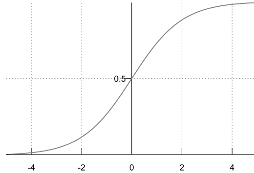
Figure 3.1 The logistic function.
