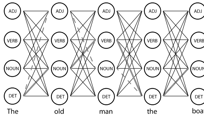
Figure 10.7 Lattice of possible tag assignments for the example sentence from Figure 10.6. For simplicity, we only show four of the possible part-of-speech tags: DET - determiner, NOUN - common noun (either singular or plural), VERB - verb (any tense), and ADJ - adjective. The thick (green) lines indicate the correct path in the lattice; the dashed (red) lines indicate the incorrect path suggested by the first interpretation of the garden-path sentence.
