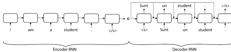
Figure 14.1 An encoder-decoder example for machine translation from English to Romanian, where both encoder and decoder are implemented using RNNs. Two virtual tokens, </s> and <s> , indicate end of sentence and beginning of sentence, respectively. The decoder uses the representation generated for the entire input sequence, i.e., the hidden state vector c of the </s> token in the English sentence, to generate the equivalent Romanian words.
