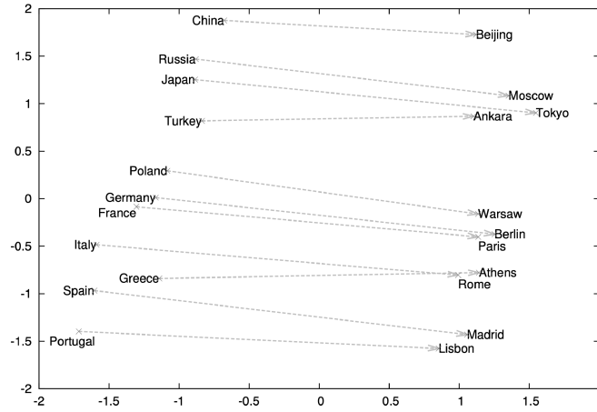
Figure 8.3 Two-dimensional projection of 1000-dimensional vectors learned by word2vec for countries and their capitals (Mikolov et al., 2013a).
