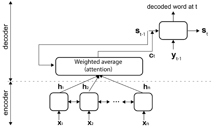
Figure 14.3 The architecture of a single decoder cell in a sequence-to-sequence architecture with attention. The encoder for this architecture is a bidirectional RNN that uses the input word embeddings, \mathbf{x}_1 to \mathbf{x}_n , to produce a sequence of hidden states, \mathbf{h}_1 to \mathbf{h}_n . The decoder is a left-to-right RNN. To avoid confusion between the source and target languages we use \mathbf{y}_t to indicate the input representation of the target word decoded at position t , and \mathbf{s}_t to indicate the hidden state produced by the decoder cell at position t . \mathbf{c}_t indicates the custom encoding vector of the source text for position t in the decoder.
