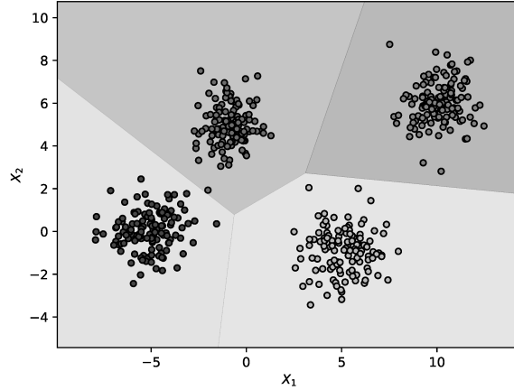
Figure 3.5 Example of a two-dimensional decision boundary for a 4-class logistic regression classifier.
