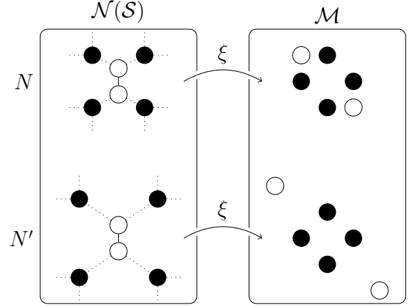
Figure 2: Graph-awareness property of a node embedding function \xi . For a given pair of nodes (labelled in white) in a network N , there is an alternative dissimilarity function that preserves their dissimilarity while expanding the dissimilarity between other pairs, yielding the network N' . The dissimilarity of the given pair under the embedding \xi is different between N and N' .
