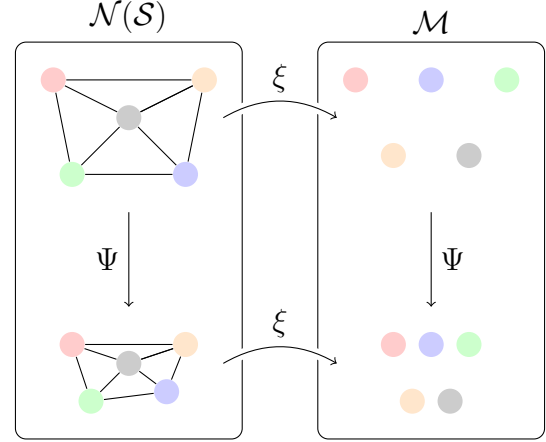
Figure 1: Consistency property of a node embedding \xi . For any two networks N_1, N_2 and a CoDNI map \Psi from N_1 to N_2 , the same map applied to their corresponding embeddings is contractive.
