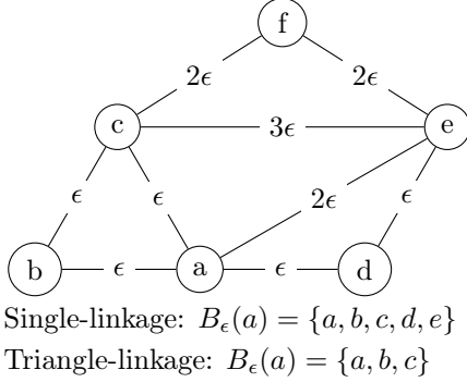
Figure 3: Single-linkage and motif-based embeddings. Pictured is a dissimilarity network on node set \{a, b, c, d, e, f\} , with dissimilarities labeled on the edges. For simplicity, assume that omitted dissimilarities in the figure take on some large value. Under the single-linkage embedding, the \epsilon -ball about the node a consists of the nodes \{a, b, c, d, e\} . In contrast, the triangle-linkage embedding only yields an \epsilon -ball about a consisting of \{a, b, c\} .
