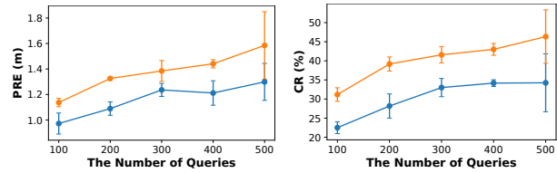
Figure 14: ATD, PRE and CR under brute-force sampling attack and our inverse attack on victim AV using AgentFormer trajectory predictor.
