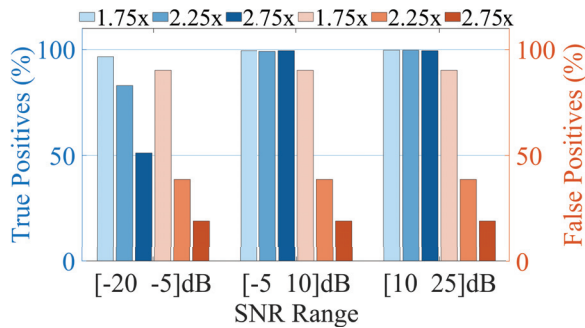
Fig. 15: Activity detection performance
