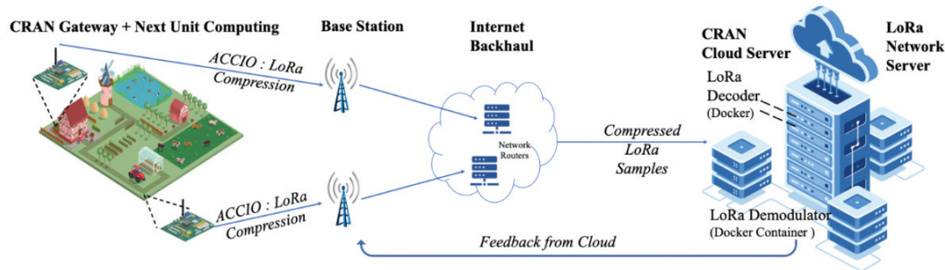
Fig. 1: An Illustration of CRAN and Cloud-LoRa
