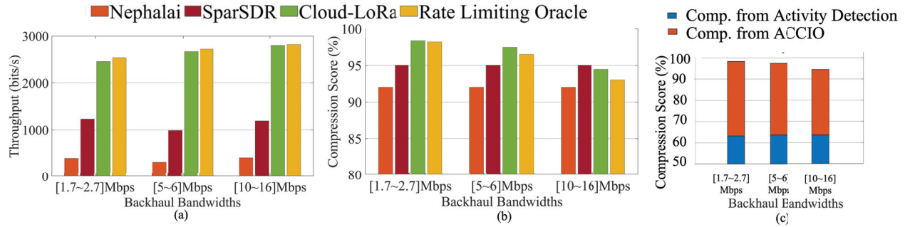
Fig. 7: (a) : Cloud-LoRa throughput performance across 8 parallel LoRa channels, averaged over multiple days in RURAL scenario. (b) Corresponding compression performance. (c) Ablation study on Compression.
