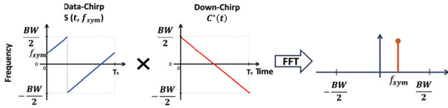
Fig. 16: LoRa Demodulation
