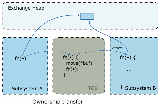
Figure 1: Private and shared heaps
