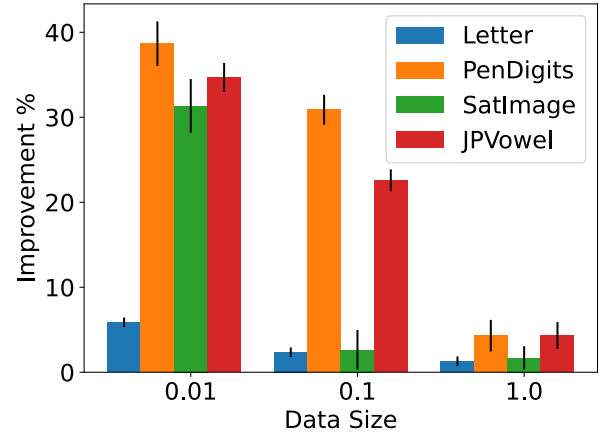
Figure 10: Same semantics as in Figure 3. Environment: binary-valued cost, \mu_{\text{good}, \epsilon=0.1} , and # actions = 5 \times # classes.
