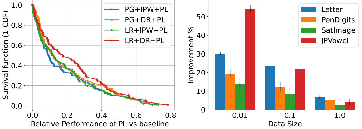
Figure 1: Relative improvement ( RelImp ) for PL against the baseline with no pessimism: mean over all runs.
