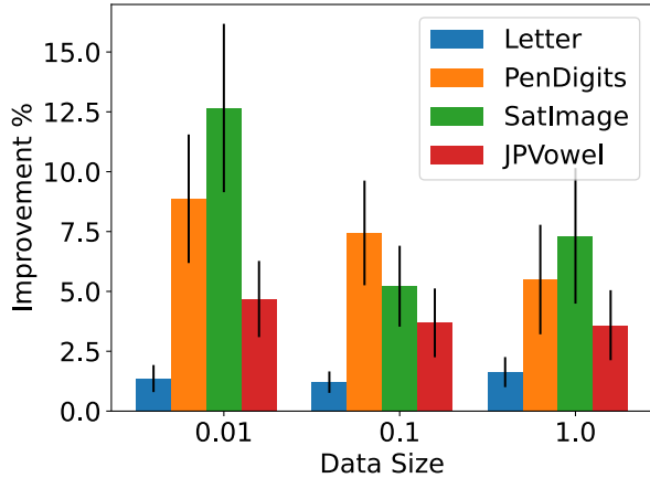
Figure 5: Same semantics as in Figure 3.
