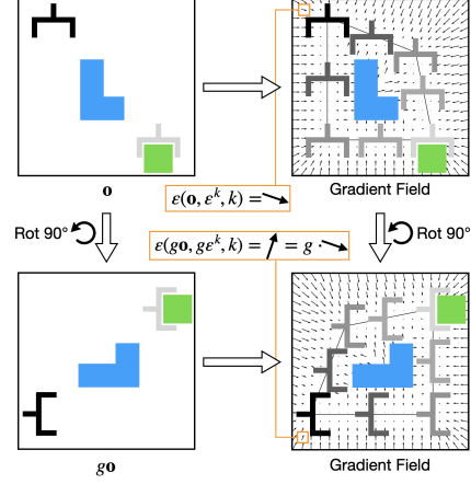
Figure 2: Equivariance of the denoising function \varepsilon . Left: In observation \mathbf{o} , the goal for the gripper is to reach the green block while avoiding the blue obstacle. Right: The expert trajectory and the gradient field associated with the denoising function. If the policy is equivariant, both the denoising function and the entire gradient field is equivariant. The orange boxes show the equivariance of \varepsilon with a particular input \varepsilon^k .
