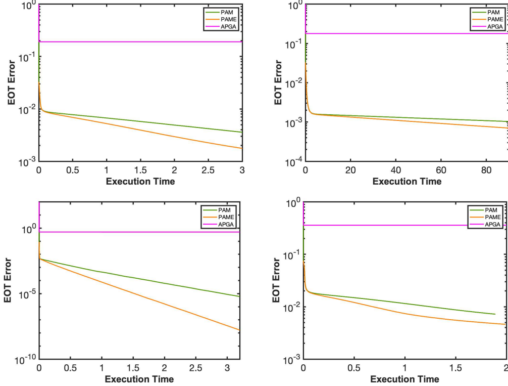
Figure 1: Computational time comparison between PAM, PAME and APGA algorithms on Gaussian distributions. Upper Left: N = 10, n = 100, \eta = 0.1 , Upper Right: N = 10, n = 500, \eta = 0.1 , Bottom Left: N = 10, n = 100, \eta = 0.5 , Bottom Right: N = 5, n = 100, \eta = 0.1 .
